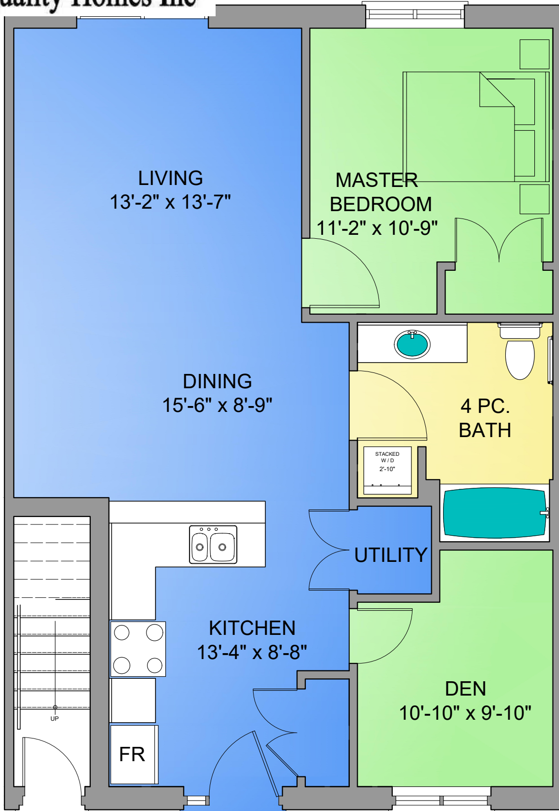
UNIT 4 & 11 FLOOR PLAN PHASE 3 872 SQ. FT. UNIT AREA
