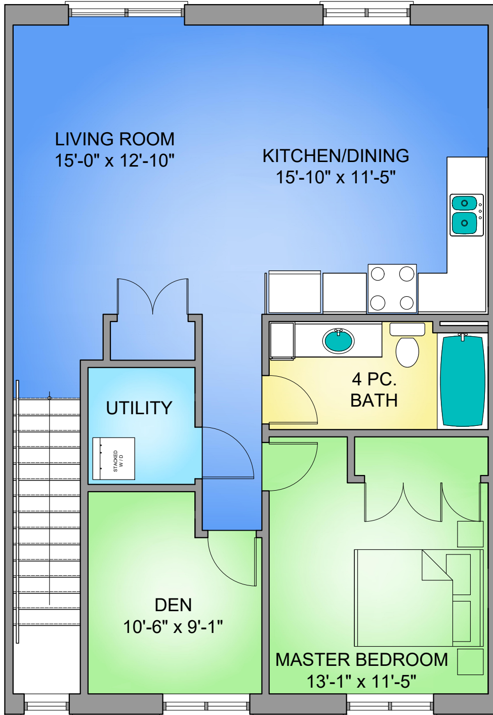
UNIT 3 & 12 FLOOR PLAN PHASE 3 931 SQ. FT. UNIT AREA
