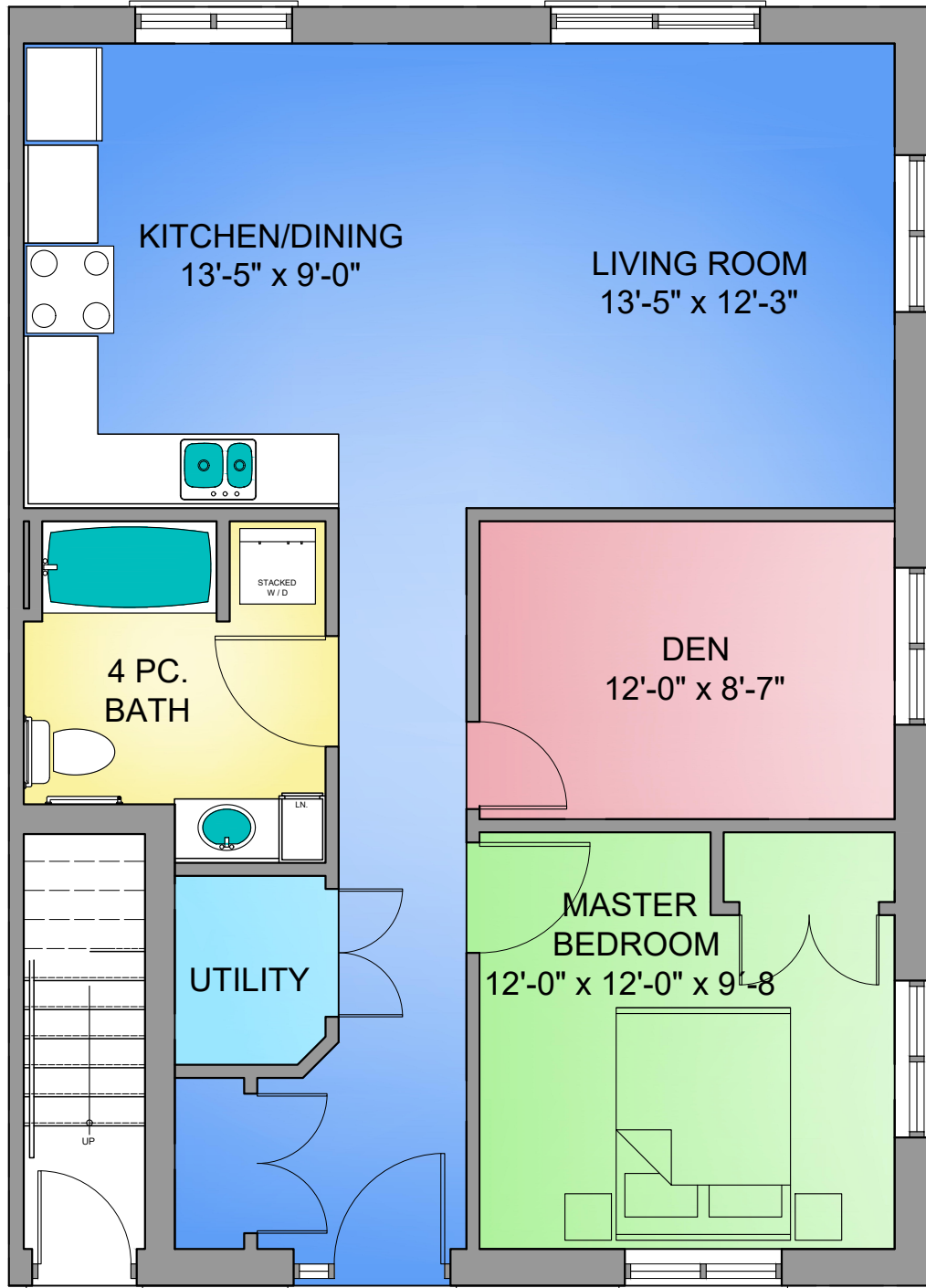
UNIT 14 FLOOR PLAN PHASE 3 912 SQ. FT. UNIT AREA
